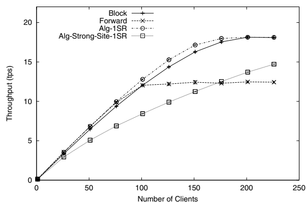
Figure 5. Transaction Throughput vs. Number of Clients
